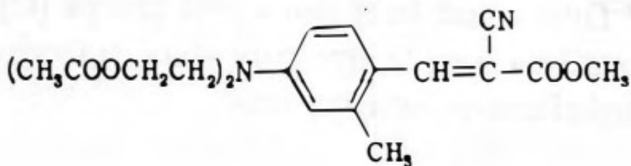
(XCVI)
