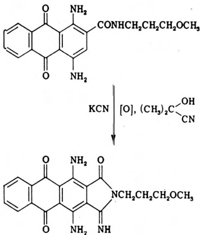
CHART 16
